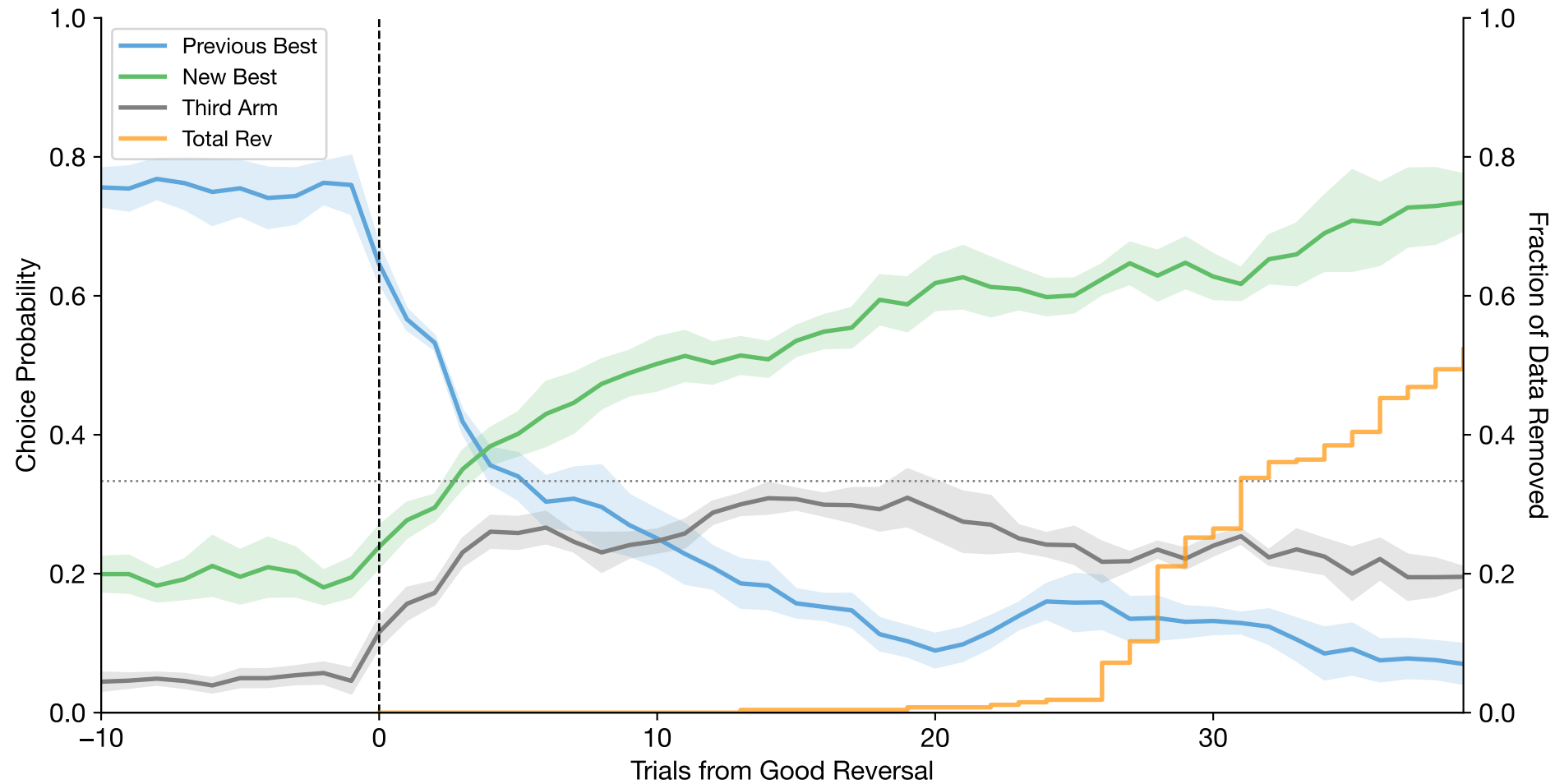
Reversal-Aligned Choices (mean \pm se across problems | n=6 subjects, n=192 reversals, n=5 problems)
